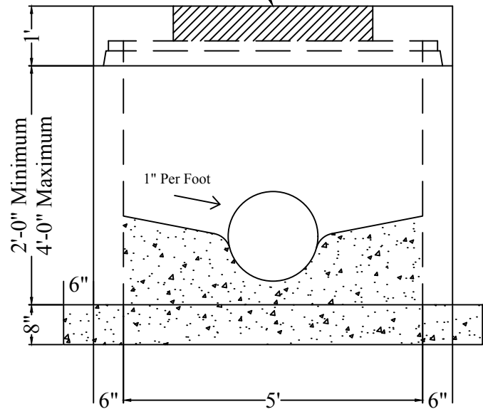
60" Manhole With Flat Lid
